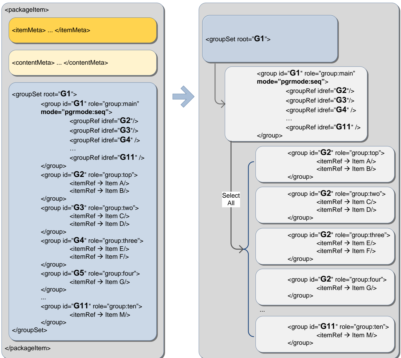
Figure 5: Code skeleton of a sequential mode package and (right) the resulting relationship structure
