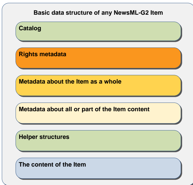
Figure 1: All G2 Items share this basic container structure
