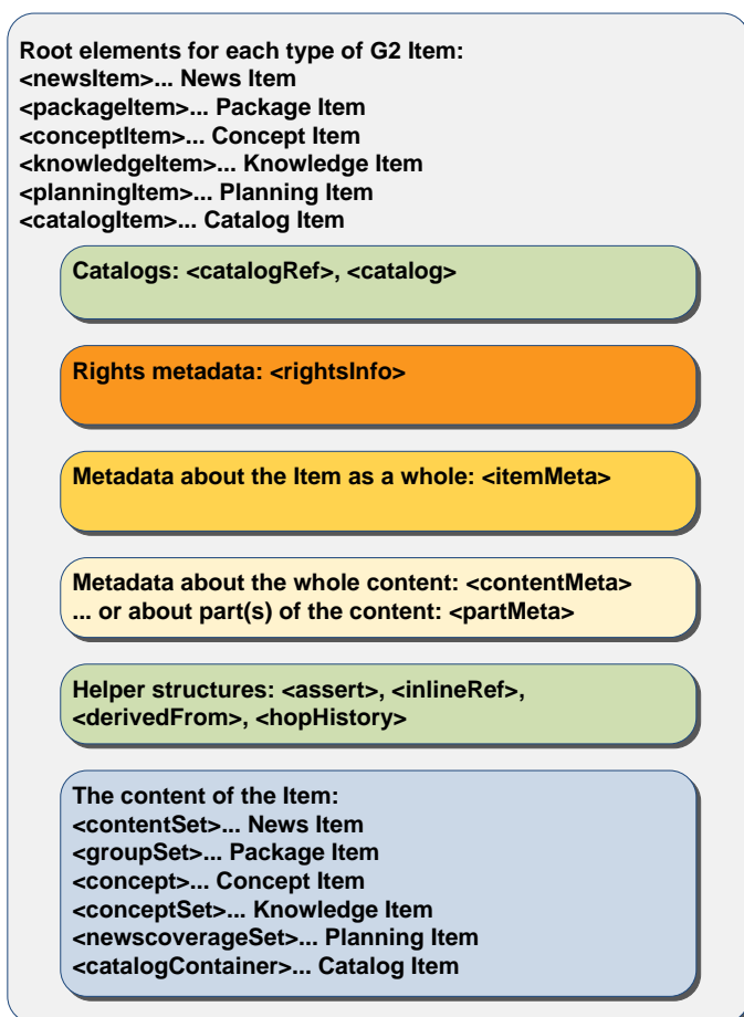
Figure 2: The basic XML elements associated with each part of a G2 Item
